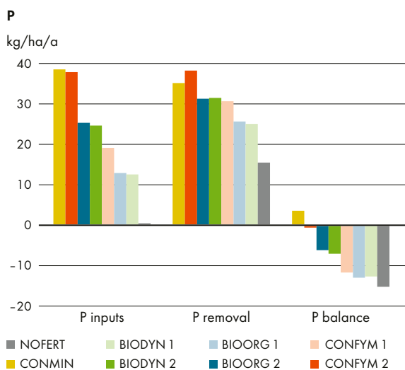
Figure 22: Phosphorus balance
